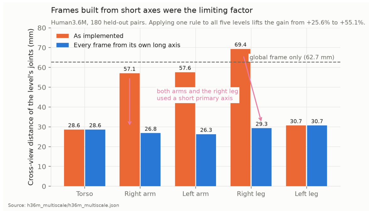
Figure 5.10: Per-level cross-view distance on Human3.6M. Three of the five frames were built from an axis roughly half a shoulder or hip width long; rebuilding them from the segment's own long axis halves their cross-view distance and brings all five levels into a 4.4 mm band.
