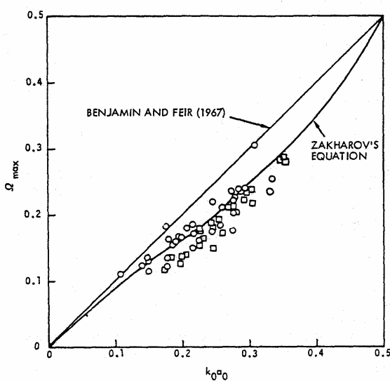
Figure 7.3 Most unstable modulation frequency \Omega_{MAX} as a function of carrier wave steepness k_0 a_0 (Yuen & Lake, 1980).
