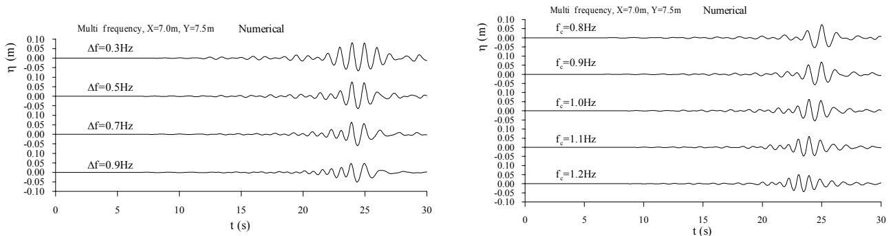
Figure I.5.3 Effects of center frequency and bandwidth on directional wave focusing efficiency.
