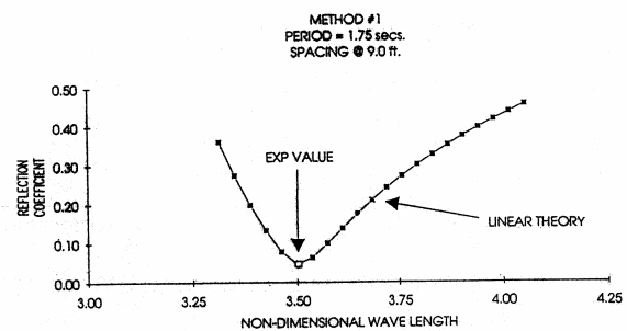
Figure 7.6 Effect of the choice of the wave number on the reflection coefficient (Cotter and Chakrabarti, 1992).
