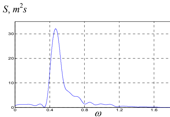
Figure I.1.6 Spectral density functions of the peak state from measured result.
