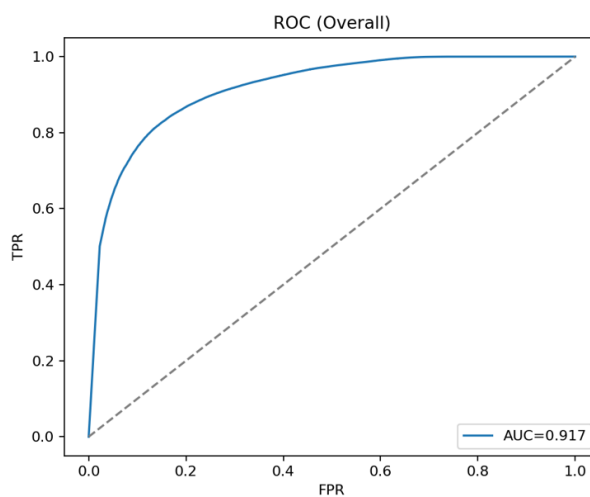
Figure G.3: HybridResNetEnvironmental ROC Curve
