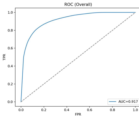
Figure G.3: HybridResNetEnvironmental ROC Curve
