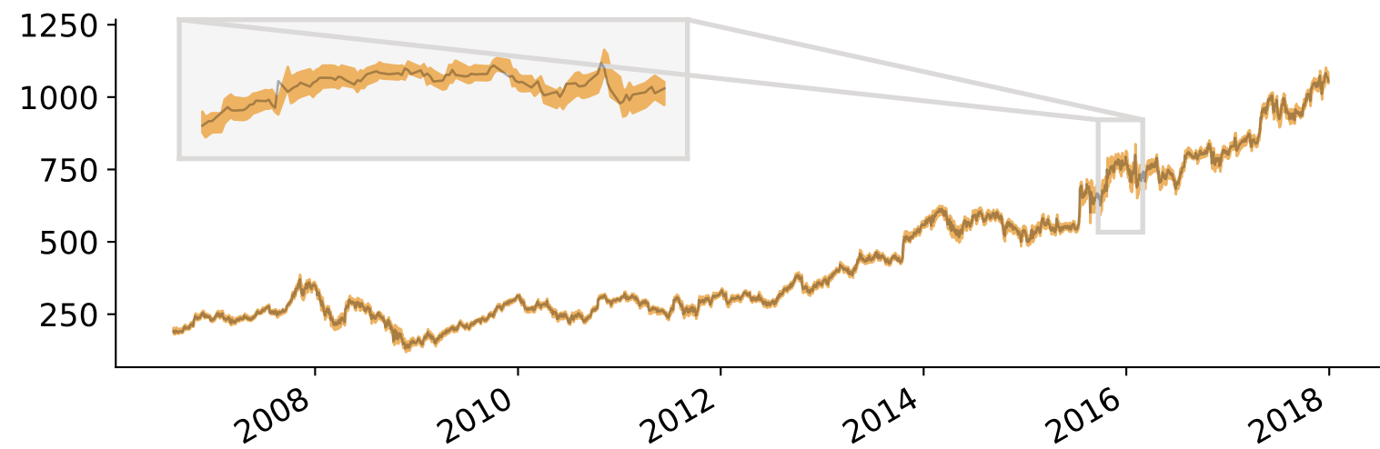
Sets
