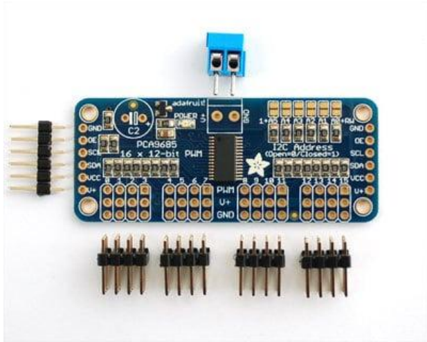
Figure 12. PCA9685 [10] servo driving board
