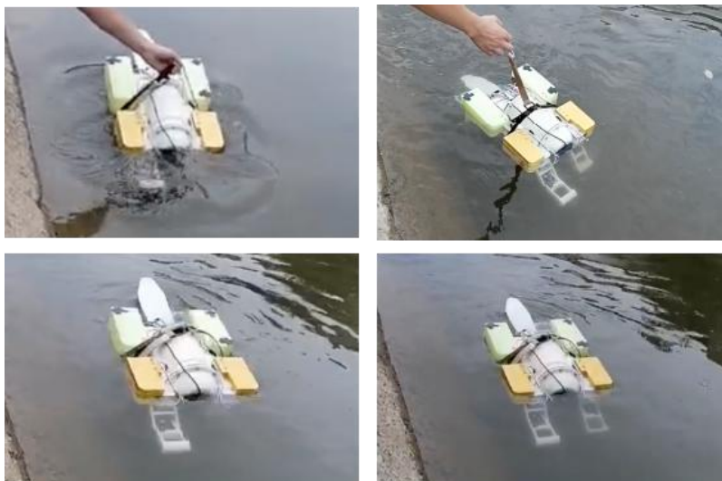
Figure 25. Outdoor swimming test
