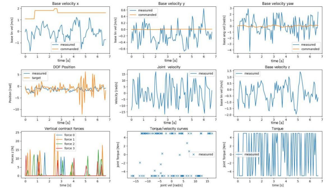
Figure 20. Issac Gym Training Result of Terrestrial Motion
