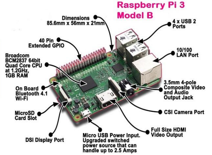
Figure 11. Raspberry Pi 3b
