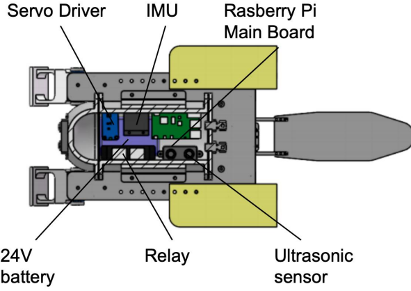
Figure 5. The Internal Distribution of The Waterproof Cabin
