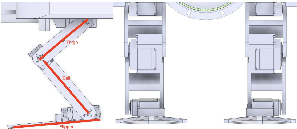
Figure 4. The Mechanical Design of The Hind Limbs(left view & front view)
