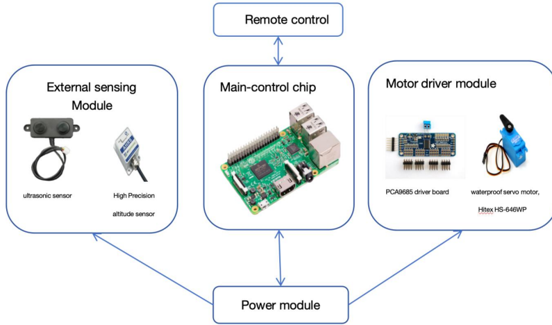
Figure 10. Hardware System Design
