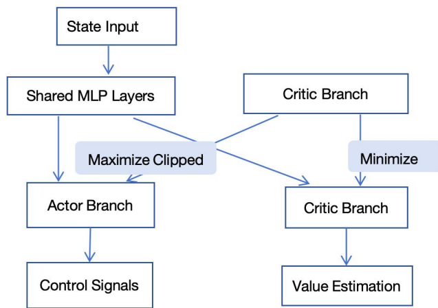
Figure 17. Neural Network Diagram
