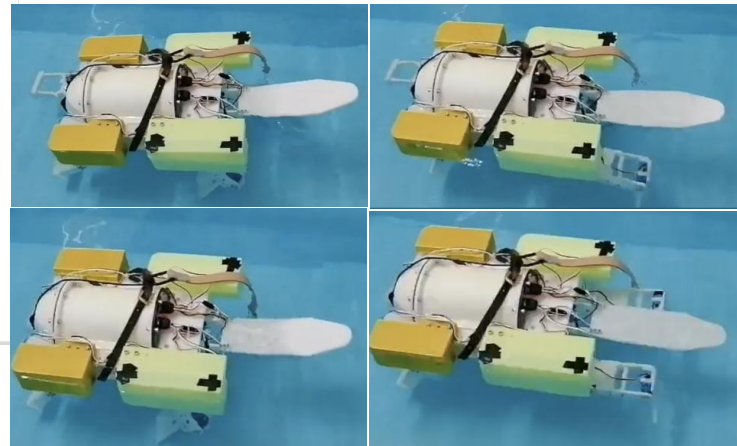
Figure 24. Real Time Robot Aquatic Locomotion Test
