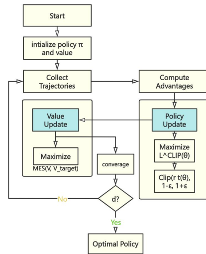
Figure 18. Flowchart based on PPO reinforcement learning
