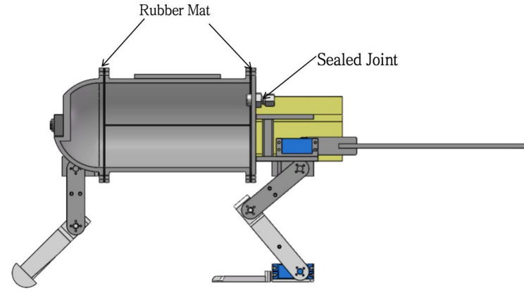
Figure 6. The Waterproof Measures on the Sealed Cabin
