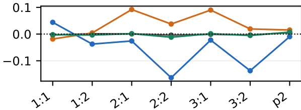
RMSE
