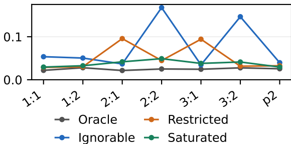
RMSE
