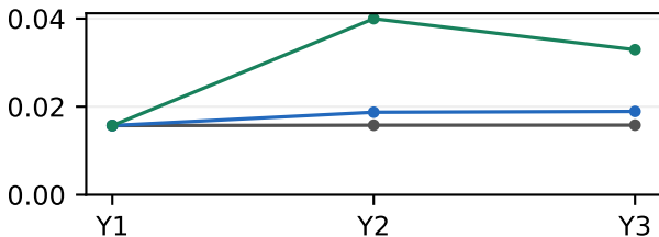
Coverage (valid)
