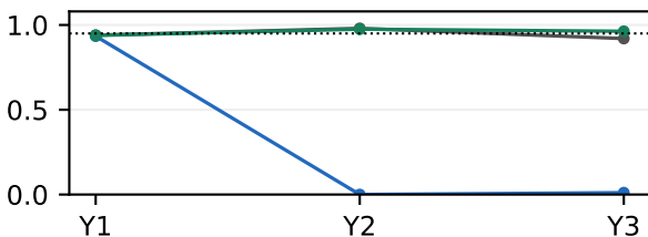
Coverage (valid)
