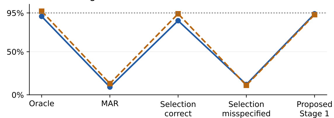
95% coverage
