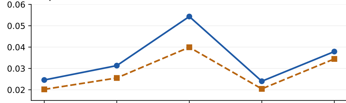
Empirical SD
