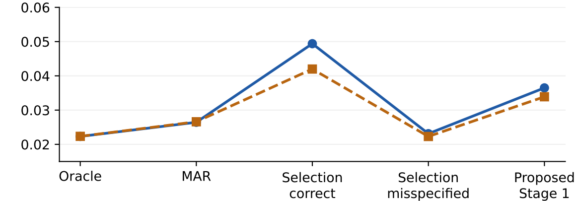
Mean estimated SE
