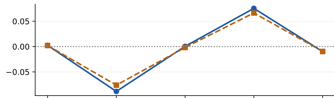
Bias
