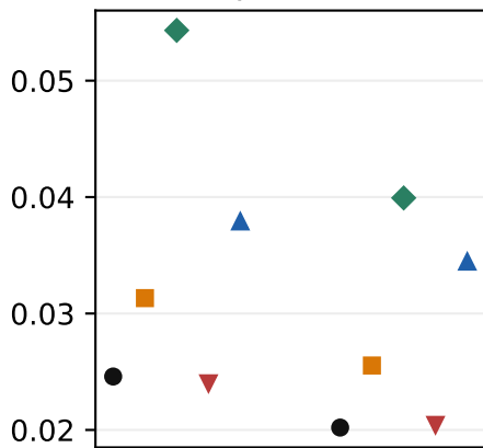
95% coverage
