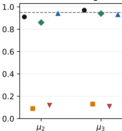
95% coverage
