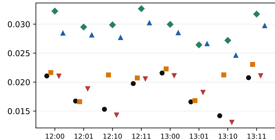
Mean estimated SE
