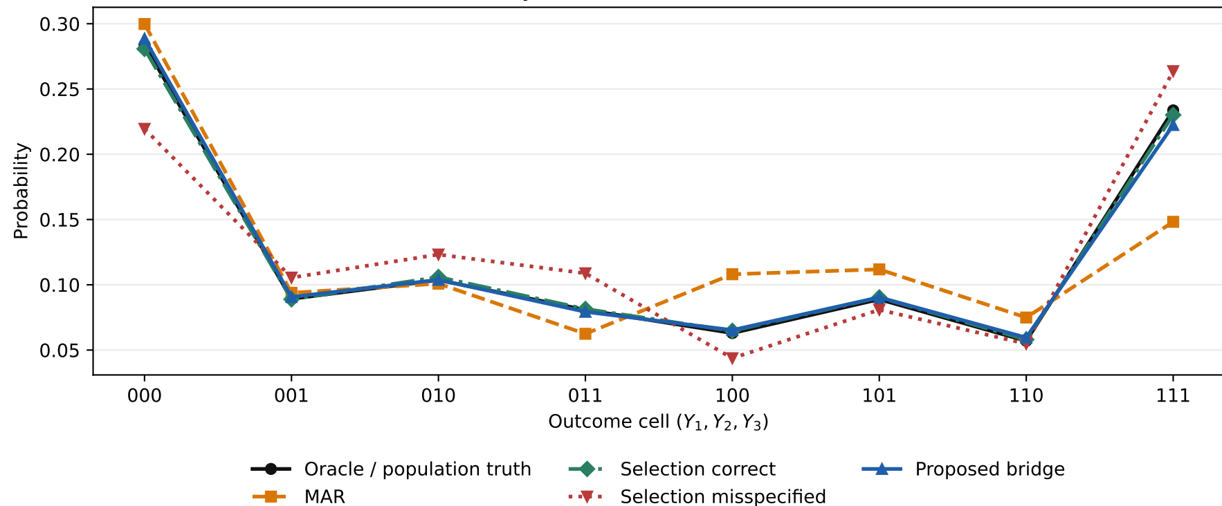
Recovery of the full outcome distribution
