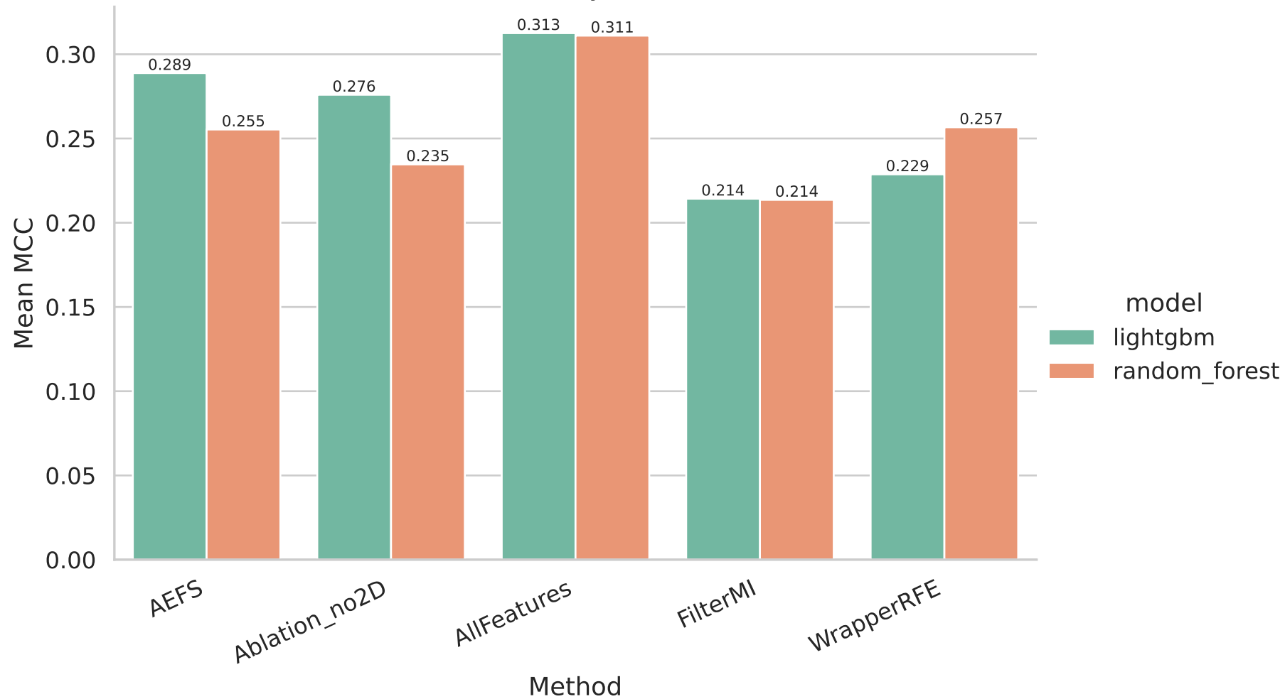
AEEEM — Mean MCC by Method and Model
