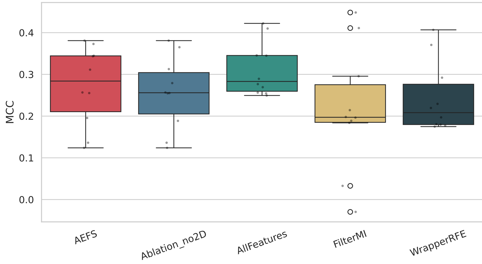
AEEEM — MCC Distribution Across LOPO Folds
