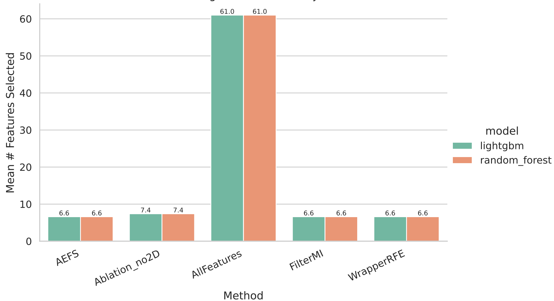
AEEEM — Average Feature Count by Method
