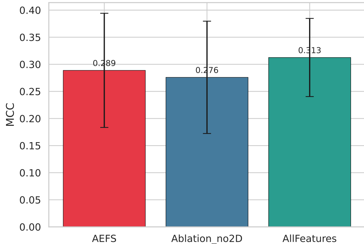
AEEEM — Ablation Study (LightGBM)
