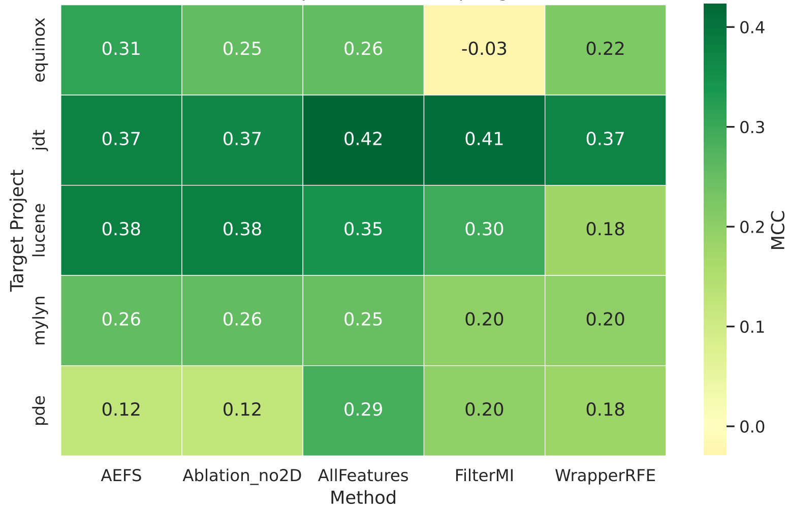
AEEEM — Per-Project MCC Heatmap (LightGBM)
