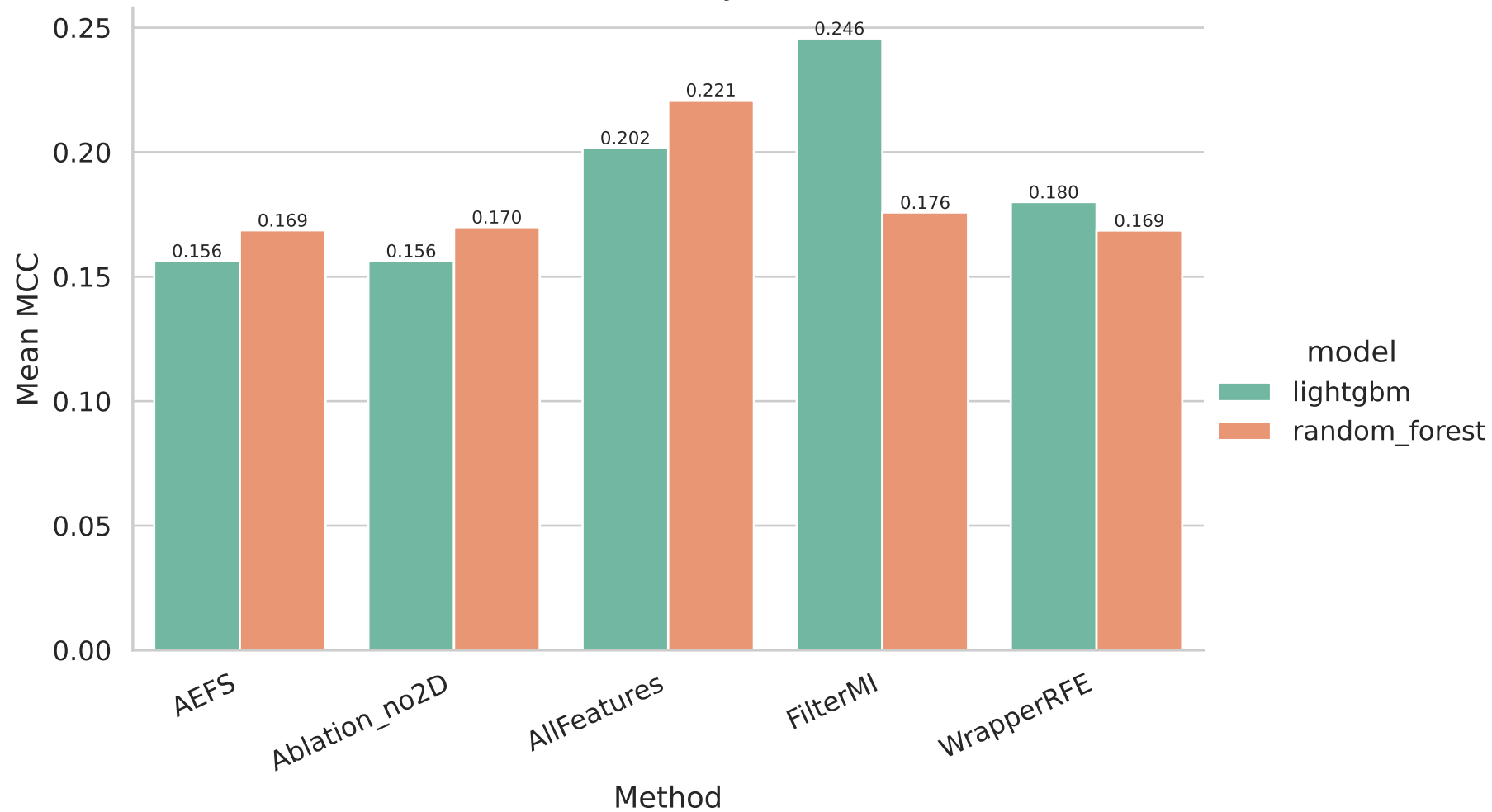
TeraPromise — Mean MCC by Method and Model
