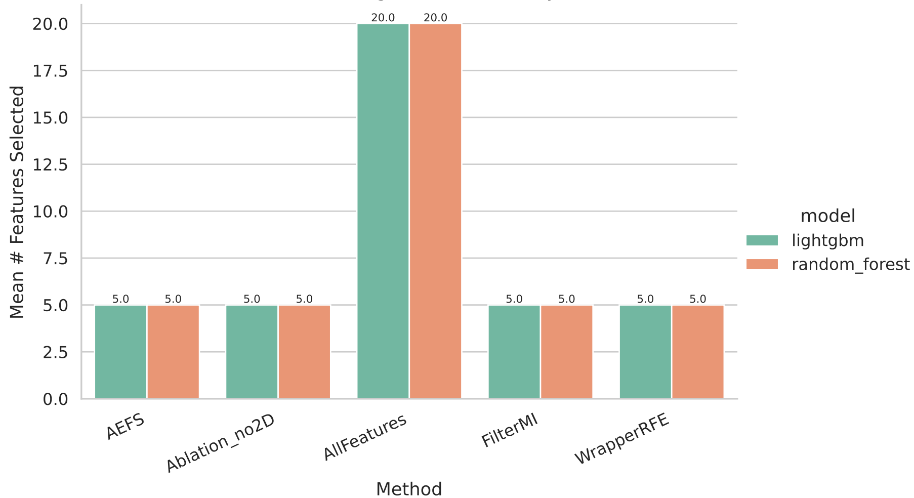
TeraPromise — Average Feature Count by Method
