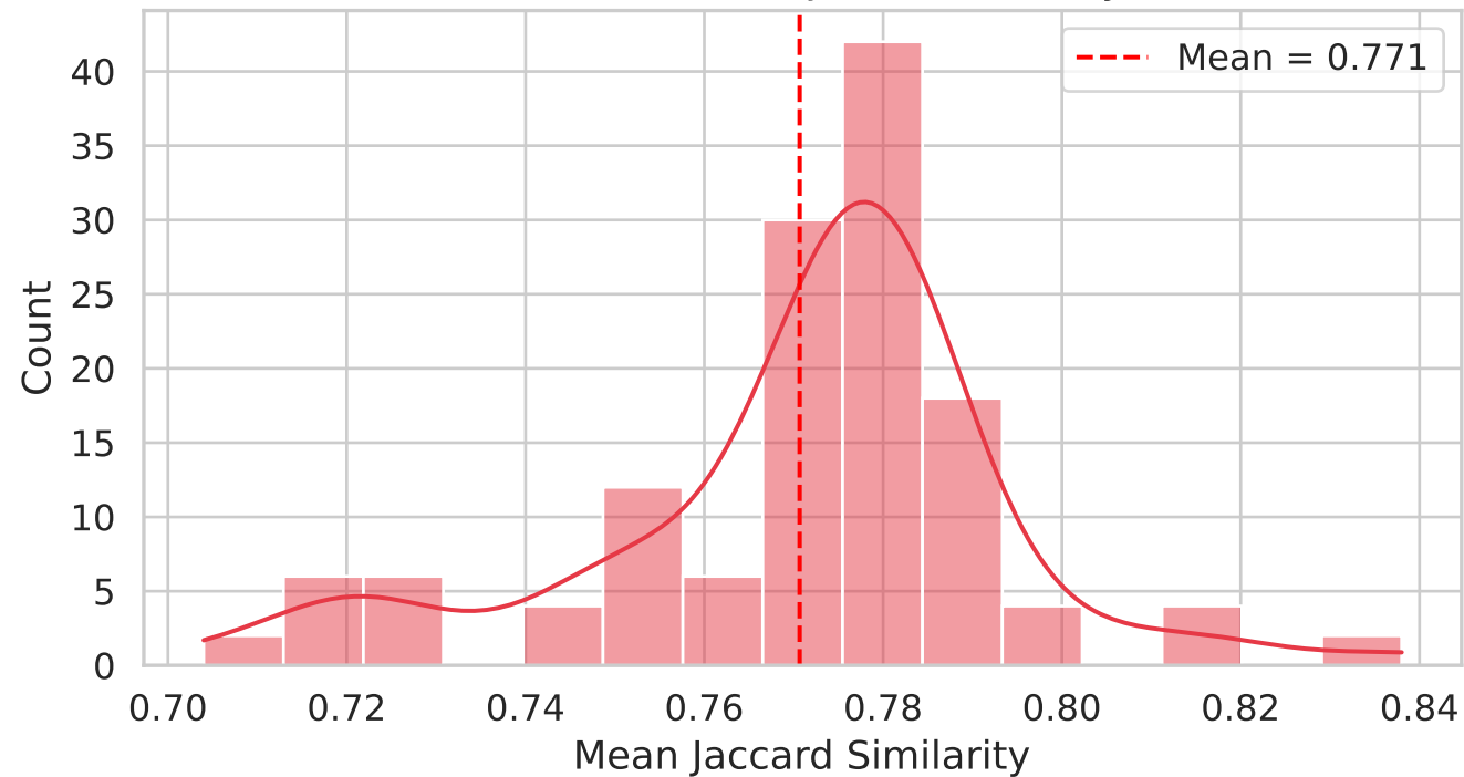
TeraPromise — Pairwise Jaccard Stability (AEFS)
