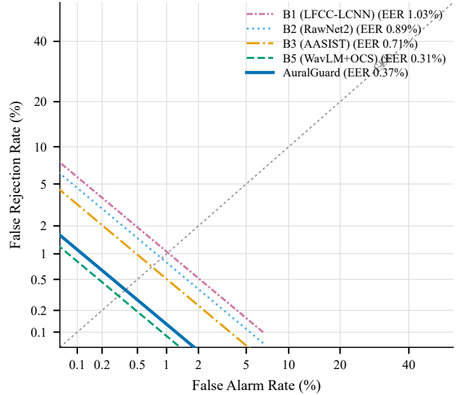
Fig. 2. DET curve comparison on the ASVspoof 2019 LA evaluation set. Curves closer to the lower-left corner are better; the dashed diagonal marks the equal-error-rate operating point. AuralGuard tracks the strong B5 baseline while clearly dominating B1–B3.
