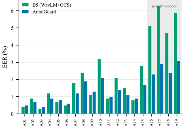
Fig. 3. Per-attack EER (%) on the ASVspoof 2019 LA evaluation set for AuralGuard versus the B5 baseline. The shaded region marks the neural-waveform attacks (A16–A19), where the vocoder-artifact branch (View B) yields the largest improvements.
