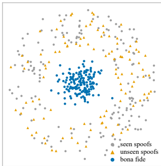
one-class contrastive (ours)
