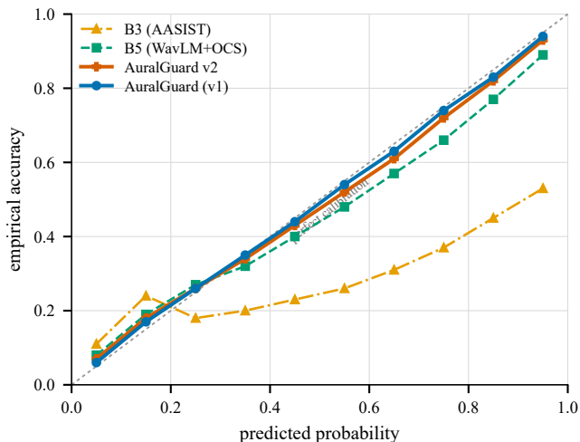
Fig. 10. Reliability diagram on the In-the-Wild benchmark evaluated zero-shot. The dashed diagonal denotes perfect empirical calibration. AuralGuard (v1) and AuralGuard v2 maintain close alignment with the identity diagonal under severe real-world domain shift ( \text{ECE} = 0.0965 and 0.1716 ), whereas B3 AASIST collapses into extreme miscalibration ( \text{ECE} = 0.5552 ).
