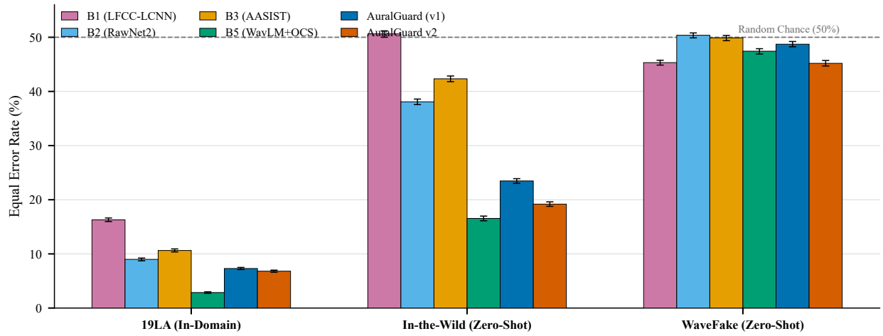
Fig. 6. Cross-corpus Equal Error Rate (%) comparison across the three benchmark evaluation domains with 95% bootstrap confidence intervals (error bars). The dashed line marks random chance performance (50% EER). Legacy acoustic architectures (B1, B2, B3) exhibit complete operational collapse on In-the-Wild and WaveFake, whereas foundation-model architectures (B5, AuralGuard) preserve strong zero-shot generalization.
