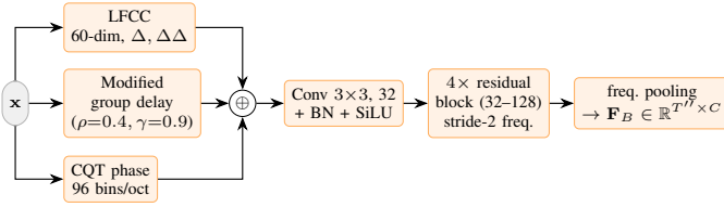
Fig. 2. View B, the vocoder-artifact branch. Three complementary time-frequency representations—magnitude cepstra (LFCC), phase-derivative structure (modified group delay), and constant-Q phase—are stacked as input channels and encoded by a light 2-D residual CNN into frame-level features \mathbf{F}_B .
