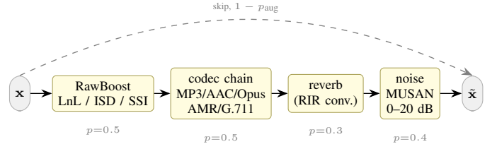
Fig. 5. Channel-robustness augmentation curriculum. Each stage is applied independently with the indicated probability; the whole pipeline is skipped with probability 1 - p_{\text{aug}} . Stage intensities are annealed from mild to full range over the first 10 epochs.
