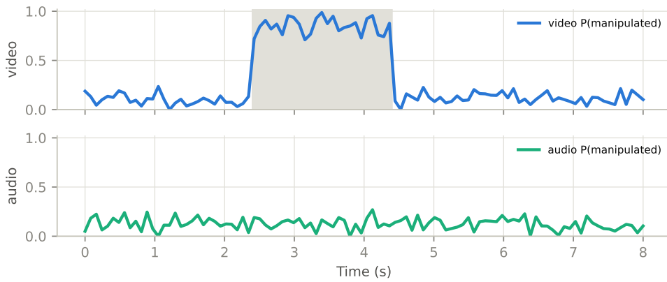
Figure 3.4: Qualitative temporal localization: per-frame manipulation probability against ground-truth manipulated intervals (shaded) (draft: demo data).
