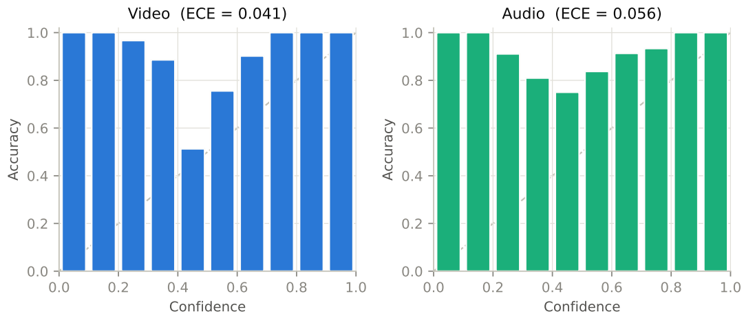
Figure 3.6: Reliability diagrams per modality with expected calibration error (draft: demo data).
