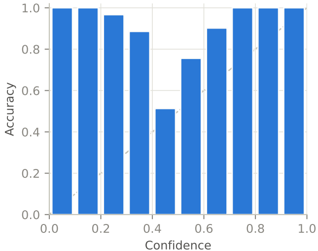
Video (ECE = 0.041)
