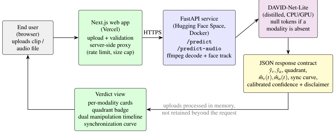
Figure 2.3: Deployment architecture. A Next.js application (Vercel) proxies uploads to a FastAPI inference service on Hugging Face Spaces running the distilled DAVID-Net-Lite; the JSON response contract carries per-modality probabilities, quadrant attribution, localization timelines, and the synchronization curve back to the verdict view.
