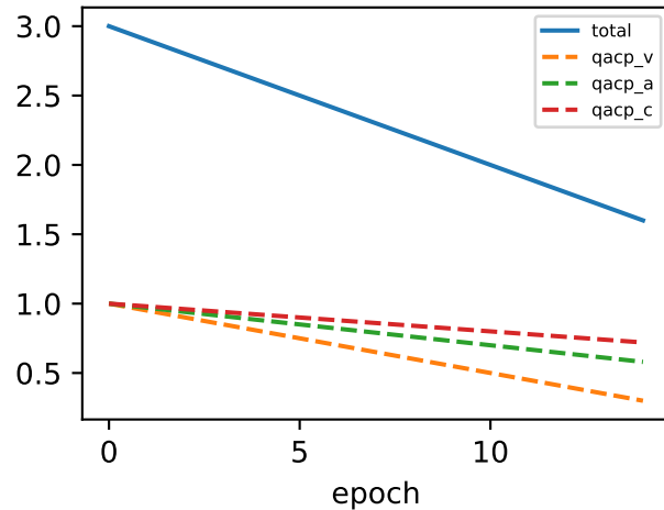
QACP (Stage 0) loss
