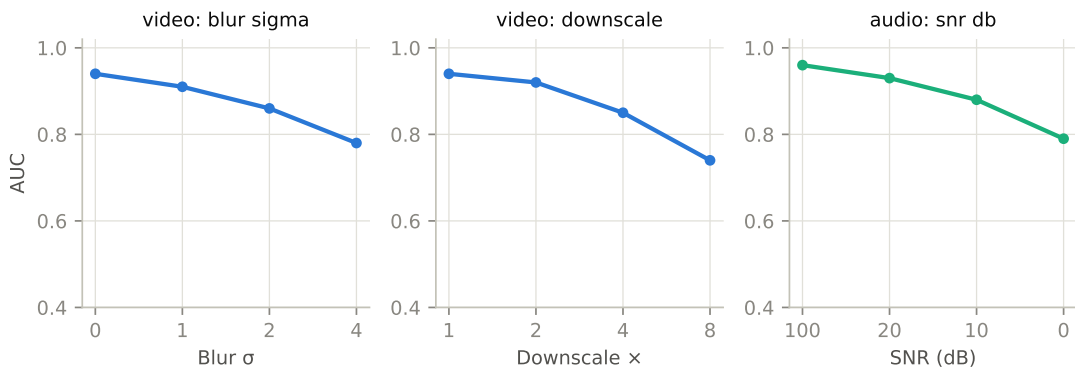
Figure 3.9: Robustness: AUC under video degradations (blur, resolution loss, quantization) and audio noise (SNR) (draft: demo data).
