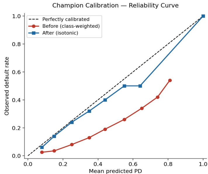
Figure 3. Reliability curve before (red) and after (blue) isotonic calibration. The calibrated curve hugs the 45° diagonal, making the PDs valid inputs to ECL = PD \times LGD \times EAD .
