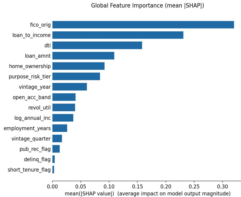
Figure 4. Global SHAP feature importance. Credit quality and affordability dominate: fico_orig (0.320), loan_to_income (0.231), dti (0.158), loan_amnt (0.109).
