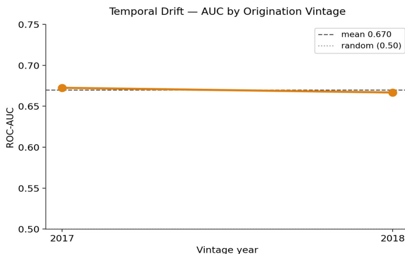
Figure 2. ROC-AUC by origination vintage on the held-out test window. Stable discrimination ( \sim 0.67 ) across cohorts is the primary evidence of production-grade generalisation.
