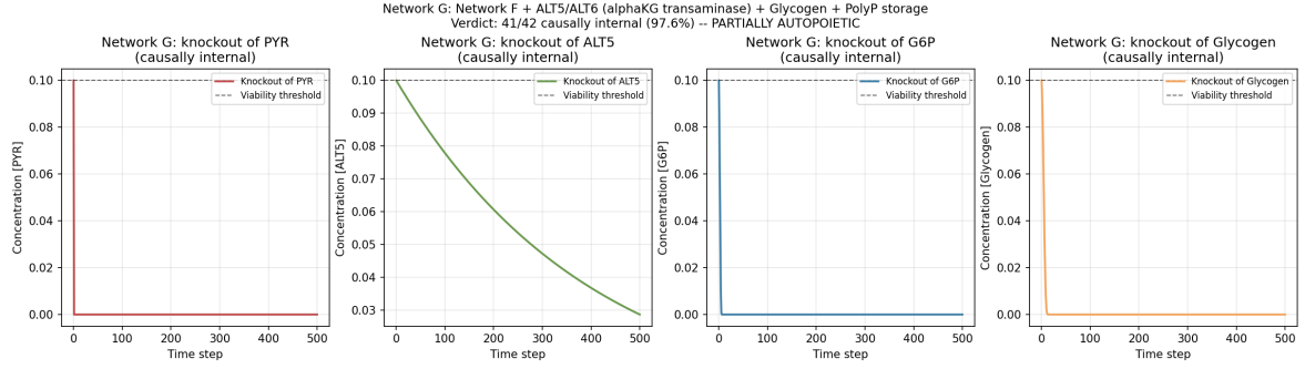
Figure 17: Network G closure-test trajectories for four representative components: PYR (cascade target broken by ALT5/6, causally internal), ALT5 (new alternative-transaminase isozyme, causally internal), G6P (metabolic intermediate buffered by Glycogen, causally internal), Glycogen (new storage compound, causally internal). Viability threshold x_{\text{thresh}} = 0.1 (dashed). Network G verdict: 41/42 causally internal (97.6%), strictly greater than Network F’s 29/31 (93.5%) in both absolute and relative terms.
