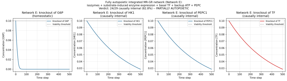
Figure 15: Autopoiesis closure test (Definition 3.18) on the fully autopoietic integrated MR-GR Network E with isozymes, substrate-induced enzyme expression, basal TF synthesis, backup ATP (ACK), and anaplerotic PEPC. Knockout trajectories for four representative components: G6P (upstream metabolic, homeostatic due to cascade collapse), HK1 (enzyme with isozyme HK2 as backup, causally internal — HK2 keeps the pathway running while HK1 is resynthesized), PEPC1 (anaplerotic enzyme with isozyme PEPC2, causally internal), and TF (regulatory, causally internal via basal constitutive synthesis). The viability threshold x_{\text{thresh}} = 0.1 (dashed). Network E verdict: 24/29 causally internal (82.8%), strictly greater than Network D’s 5/17 (29.4%) in both absolute and relative terms.
