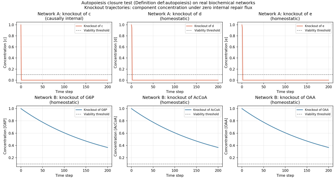
Figure 13: Autopoiesis closure test (Definition 3.18) on two real biochemical networks. Top row: Network A (Hordijk–Steel RAF); knockout trajectories of components c , d , e under zero internal repair flux with food supply held fixed and degradation active. Bottom row: Network B ( E. coli core metabolism); knockout trajectories of G6P, AcCoA, OAA. Viability threshold x_{\text{thresh}} = 0.1 (dashed). Components whose trajectories recover above the threshold after restoration of the repair pathway are AUTOPOIETIC; those that remain at 0 are HOMEOSTATIC. Network A: 2/5 causally internal; Network B: 0/10 causally internal.
