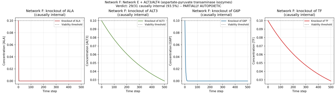
Figure 16: Autopoiesis closure test (Definition 3.18) on Network F: Network E + ALT3/ALT4 aspartate-pyruvate transaminase isozymes (EC 2.6.1.12) with ASP-based synthesis. Knockout trajectories for four representative components: ALA (cascade target, now causally internal — ALT3/ALT4 produce ALA via M11 during recovery), ALT3 (new enzyme, causally internal — its synthesis uses ASP not ALA, so it stays at high level even during ALA knockout), G6P (upstream metabolic, still homeostatic due to remaining cascade), TF (regulatory, causally internal). Viability threshold x_{\text{thresh}} = 0.1 (dashed). Network F verdict: 29/31 causally internal (93.5%), strictly greater than Network E’s 24/29 (82.8%) in both absolute and relative terms.
