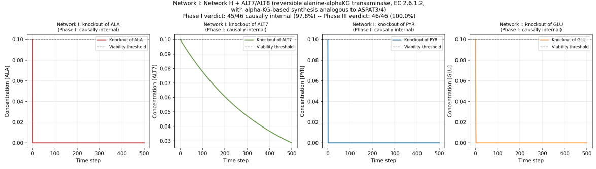
Figure 19: Network I closure-test trajectories for four representative components: ALA (cascade target of ALT7/8, the limit-cycle that is now DAMPENED and causally internal at Phase I), ALT7 (new reversible alanine transaminase isozyme with \alpha KG-based synthesis, causally internal), PYR (substrate of M19 ; causally internal at Phase I), GLU (substrate of M19 ; alternative ALA substrate, causally internal). Viability threshold x_{\text{thresh}} = 0.1 (dashed). Network I Phase I verdict: 45/46 causally internal (97.8%), strictly greater than Network H’s 43/44 (97.7%) in both absolute and relative terms. Network I Phase III (pathwise + univalence-corrected) verdict: 46/46 = 100%.
