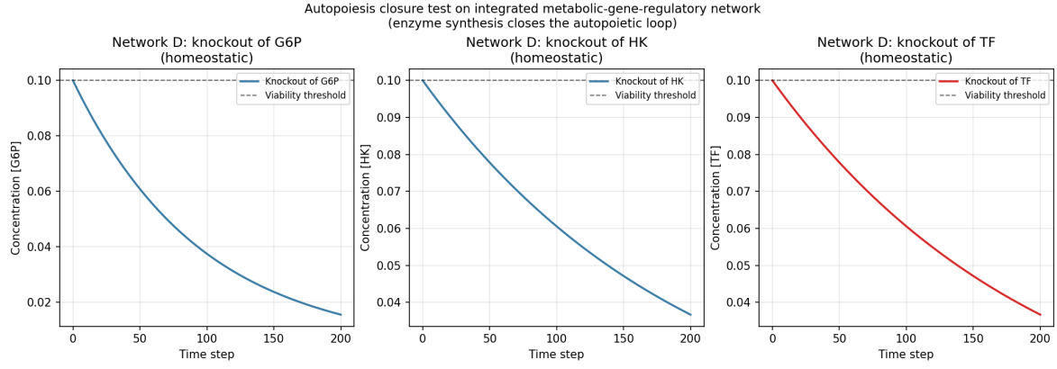
Figure 14: Autopoiesis closure test (Definition 3.18) on the integrated metabolic-gene-regulatory Network D. Knockout trajectories for three representative components: G6P (metabolic intermediate, homeostatic), HK (enzyme, homeostatic), TF (regulatory, homeostatic). The viability threshold x_{\text{thresh}} = 0.1 (dashed). None of the three representatives recovers above the threshold after restoration of the repair pathway, but other components (AcCoA, ASP, MAL, ASPAT, MDH) do recover, giving the partial-autopoiesis verdict (5/17 causally internal).
