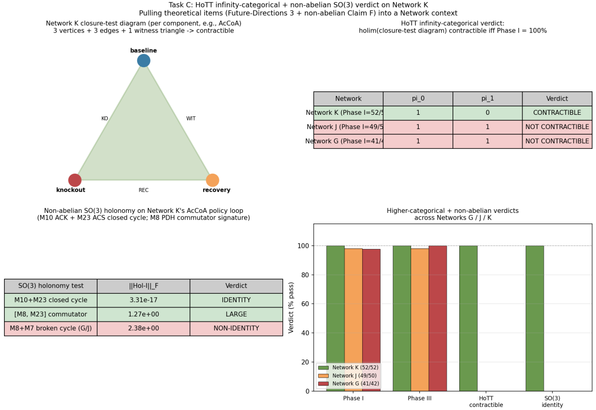
Figure 22: Higher-categorical and non-abelian verdicts on Network K. (Top-left) Per-component closure-test diagram (3 vertices + 3 edges + 1 witness triangle = topological disk = contractible per PASS component); (top-right) HoTT contractibility table across Networks K/J/G (contractible iff Phase I = 100%, Proposition 18.26); (bottom-left) non-abelian \mathfrak{so}(3) holonomy tests: closed cycle (M10+M23) identity \|\text{Hol} - I_3\|_F = 3.3 \times 10^{-17} ; commutator [M8, M23] detectable non-abelian signature \|\cdot - I_3\|_F = 1.27 ; broken cycle (M8+M7) of Networks G/J non-identity \|\text{Hol} - I_3\|_F = 2.38 (Proposition 18.28); (bottom-right) cross-network verdict bar chart showing Phase I, Phase III, HoTT-contractible, and SO(3)-identity verdicts across Networks G/J/K.
