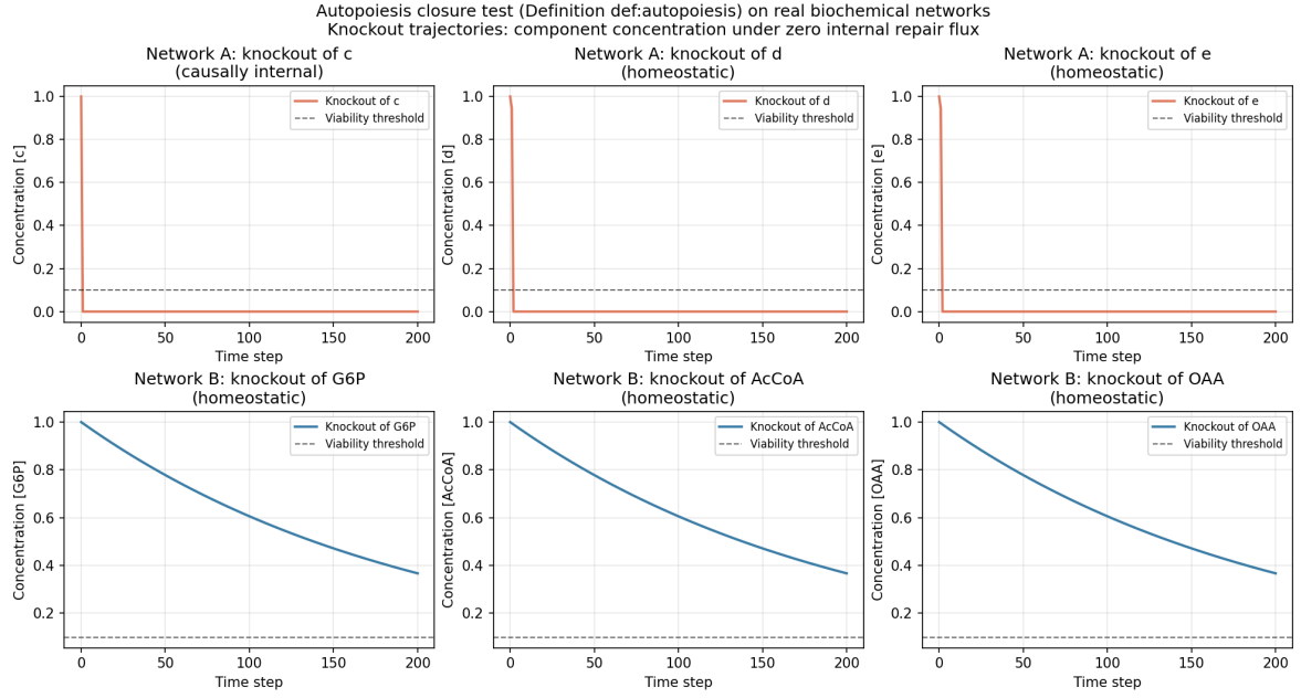
Figure 14: Autopoiesis closure test (Definition 3.18) on two real biochemical networks. Top row: Network A (Hordijk–Steel RAF); knockout trajectories of components c , d , e under zero internal repair flux with food supply held fixed and degradation active. Bottom row: Network B ( E. coli core metabolism); knockout trajectories of G6P, AcCoA, OAA. Viability threshold x_{\text{thresh}} = 0.1 (dashed). Components whose trajectories recover above the threshold after restoration of the repair pathway are AUTOPOIETIC; those that remain at 0 are HOMEOSTATIC. Network A: 2/5 causally internal; Network B: 0/10 causally internal.
