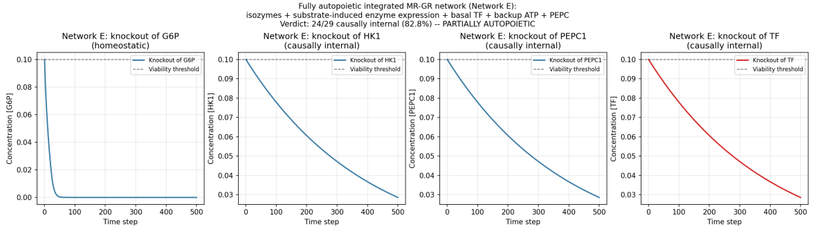
Figure 15: Autopoiesis closure test (Definition 3.15) on the fully autopoietic integrated MR-GR Network E with isozymes, substrate-induced enzyme expression, basal TF synthesis, backup ATP (ACK), and anaplerotic PEPC. Knockout trajectories for four representative components: G6P (upstream metabolic, homeostatic due to cascade collapse), HK1 (enzyme with isozyme HK2 as backup, causally internal — HK2 keeps the pathway running while HK1 is resynthesized), PEPC1 (anaplerotic enzyme with isozyme PEPC2, causally internal), and TF (regulatory, causally internal via basal constitutive synthesis). The viability threshold x_{\text{thresh}} = 0.1 (dashed). Network E verdict: 24/29 causally internal (82.8%), strictly greater than Network D’s 5/17 (29.4%) in both absolute and relative terms.
