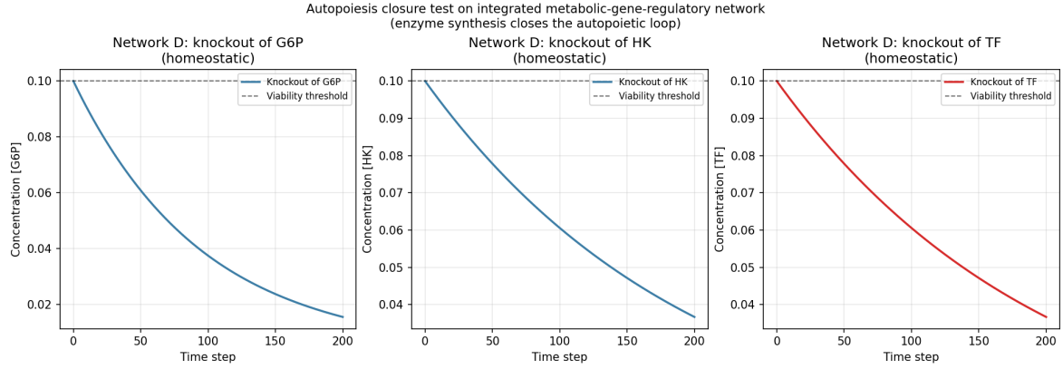
Figure 14: Autopoiesis closure test (Definition 3.15) on the integrated metabolic-gene-regulatory Network D. Knockout trajectories for three representative components: G6P (metabolic intermediate, homeostatic), HK (enzyme, homeostatic), TF (regulatory, homeostatic). The viability threshold x_{\text{thresh}} = 0.1 (dashed). None of the three representatives recovers above the threshold after restoration of the repair pathway, but other components (AcCoA, ASP, MAL, ASPAT, MDH) do recover, giving the partial-autopoiesis verdict (5/17 causally internal).
