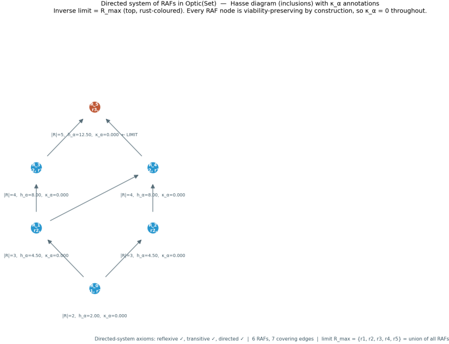
Figure 7: Hasse diagram of the directed system of RAFs in Optic (Set) over the molecule set M = \{a, b, c, d, e, f, g\} with food F = \{a, b\} and five reactions. Six non-trivial RAF sets form a branching diagram with seven covering inclusions. Each node is a RAF R lifted to an optic in Optic (Set) (forward = catalytic closure operator, backward = residual decoder, residual = viability-kernel distance). The directed-system axioms (reflexivity, transitivity, directedness) are verified by direct computation; the inverse limit equals the maximal RAF R_{\max} = \{r_1, \dots, r_5\} .
