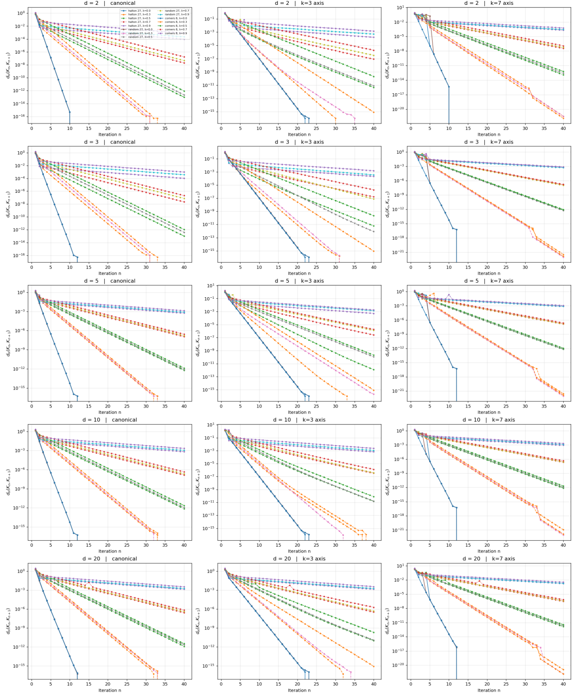
Figure 6: Robustness sweep along the dimensional axis d \in \{2, 3, 5, 10, 20\} (rows) and the axis-aligned expansion profiles canonical , k=3 axis , k=7 axis (columns). Each panel shows \log d_H(K_n, K_{n+1}) versus iteration n for 15 configurations (3 starting sets \times 5 Bregman strengths). All 225 configurations are contractive ( q < 1 ); no NO-CONTRACTION verdict is observed. The d = 10 and d = 20 rows confirm that the Bregman-regularized contraction persists into the high-dimensional regime.
