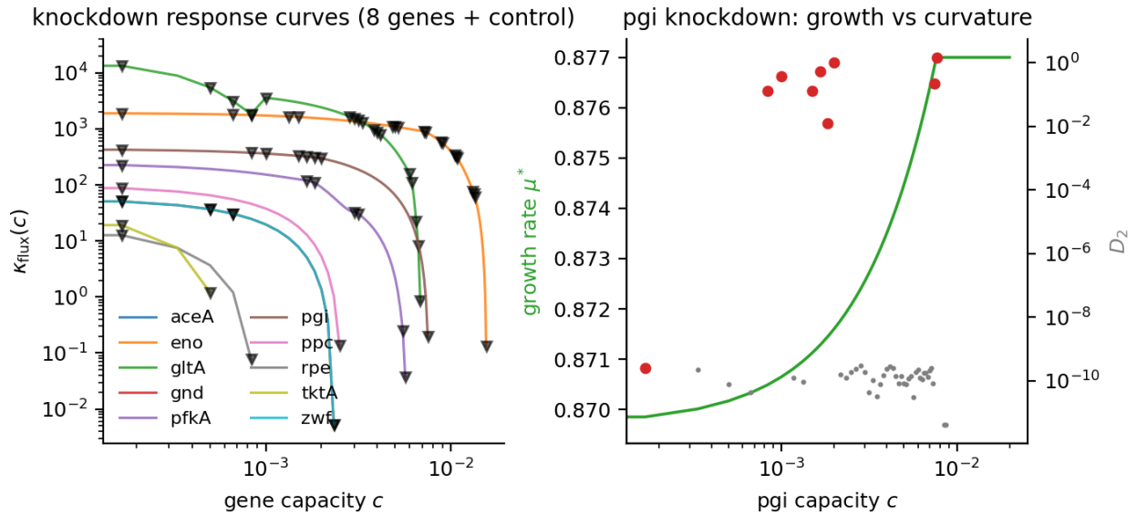
Figure 3. Left: knockdown response curves \kappa^0 \text{ flux}(c) for the gene panel (log-log; black triangles mark active-set events; aceA is the flat control). Right: pgi detail — growth (green) vs D_2 (log scale, red events).
