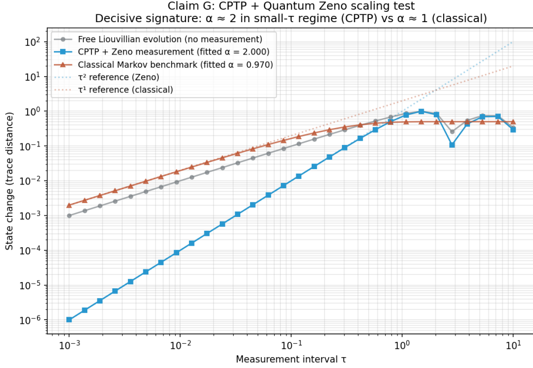
Figure 8: Quantum Zeno scaling confirmation. Log-log plot of state change (trace distance) versus measurement interval \tau . CPTP+Zeno points (blue squares) follow the \tau^2 reference line in the small- \tau regime; the fitted exponent is \alpha_{\text{Zeno}} = 1.9997 with R^2 = 1.0000 . Classical Markov points (rust triangles) follow the \tau^1 reference line; the fitted exponent is \alpha_{\text{cl}} = 0.9695 with R^2 = 0.9997 . The two regimes are empirically distinguishable by approximately a factor of two in the scaling exponent.
