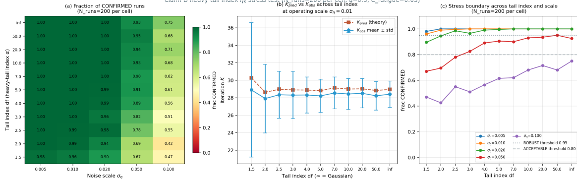
Figure 5: Heavy-tail index stress test of Claim D across the (\text{df}, \sigma_\eta) grid with N_{\text{runs}} = 200 Monte-Carlo seeds per cell. (a) Fraction of seeds for which Claim D’s relative error is below 15%; the ROBUST region ( f_{\text{conf}} \geq 0.95 , green) covers the operating scale \sigma_\eta = 0.01 across all \text{df} \geq 2 . (b) K_{\text{pred}} and K_{\text{obs}} vs. tail index at \sigma_\eta = 0.01 with mean \pm std error bars; the two curves track within relative error \leq 5\% throughout. (c) Stress boundary: f_{\text{conf}} vs. \text{df} for each \sigma_\eta ; the ROBUST threshold (0.95, dotted) and ACCEPTABLE threshold (0.80, dashed) bracket the operating regime. The infinite-variance boundary \text{df} = 2 is crossed smoothly.
