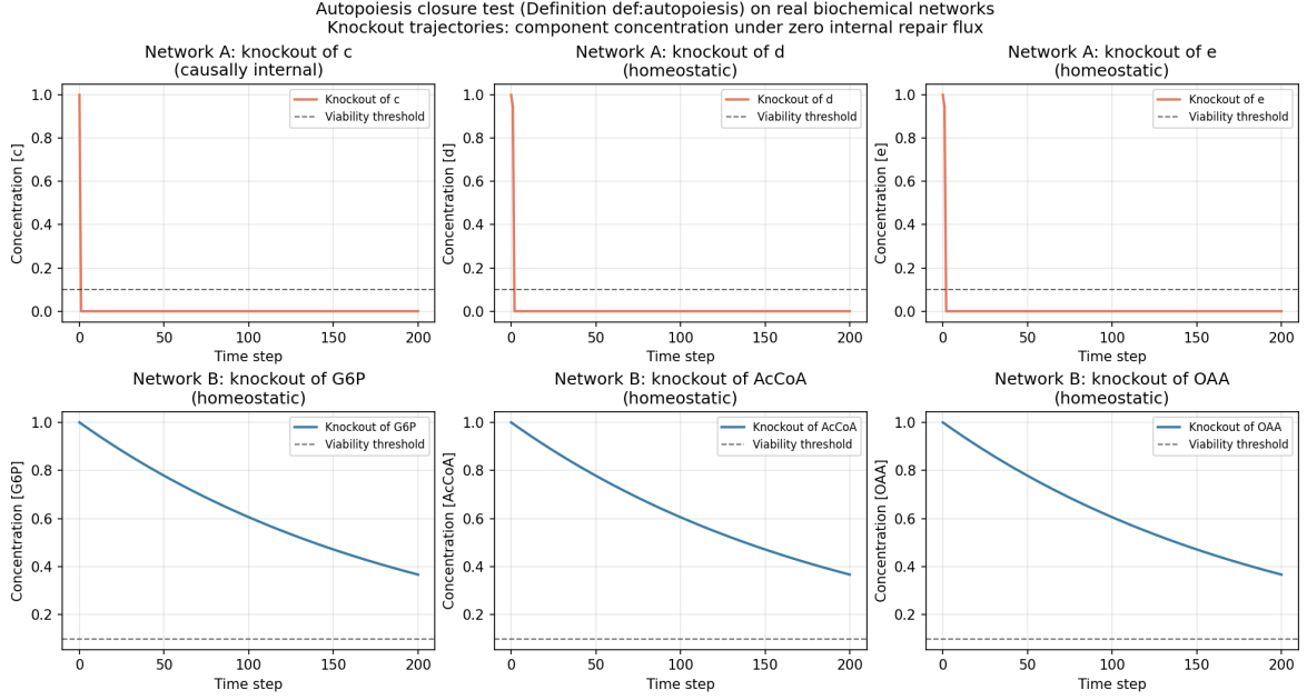
Figure 13: Autopoiesis closure test (Definition 3.10) on two real biochemical networks. Top row: Network A (Hordijk–Steel RAF); knockout trajectories of components c , d , e under zero internal repair flux with food supply held fixed and degradation active. Bottom row: Network B ( E. coli core metabolism); knockout trajectories of G6P, AcCoA, OAA. Viability threshold x_{\text{thresh}} = 0.1 (dashed). Components whose trajectories recover above the threshold after restoration of the repair pathway are AUTOPOIETIC; those that remain at 0 are HOMEOSTATIC. Network A: 2/5 causally internal; Network B: 0/10 causally internal.
