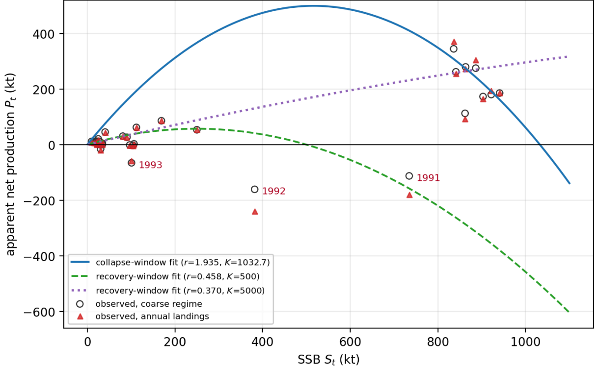
Figure 4: Apparent net production P_t = S_{t+1} - S_t + C_t against S_t under both catch treatments, with the fitted collapse-window and the two recovery-window Schaefer curves overlaid. P_t is a diagnostic construct, not a closed biomass budget: it inherits any error in the catch reconstruction and any assessment revision in the SSB series, and it is not a mass balance. The 1991–1993 points lie below every fitted curve under both treatments, and the two recovery-window parameterisations are almost indistinguishable over the observed range of S_t while diverging widely when extrapolated beyond it.
