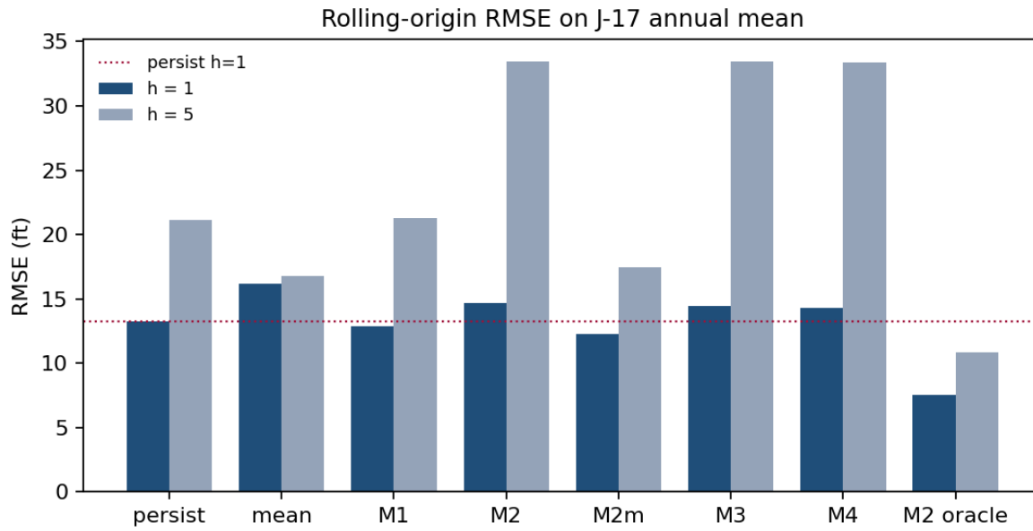
Figure 3. Rolling-origin RMSE. The oracle is excluded from retention.
