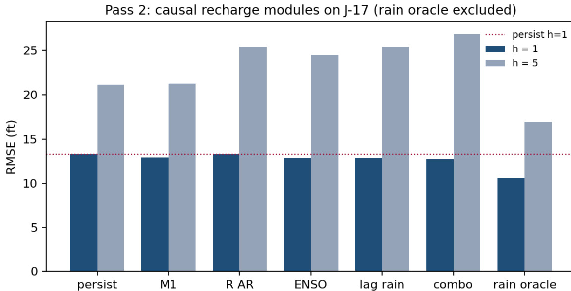
Figure 4. Rolling RMSE on J-17 for climate-informed recharge. The precipitation oracle uses year t+h precipitation and cannot be retained.
