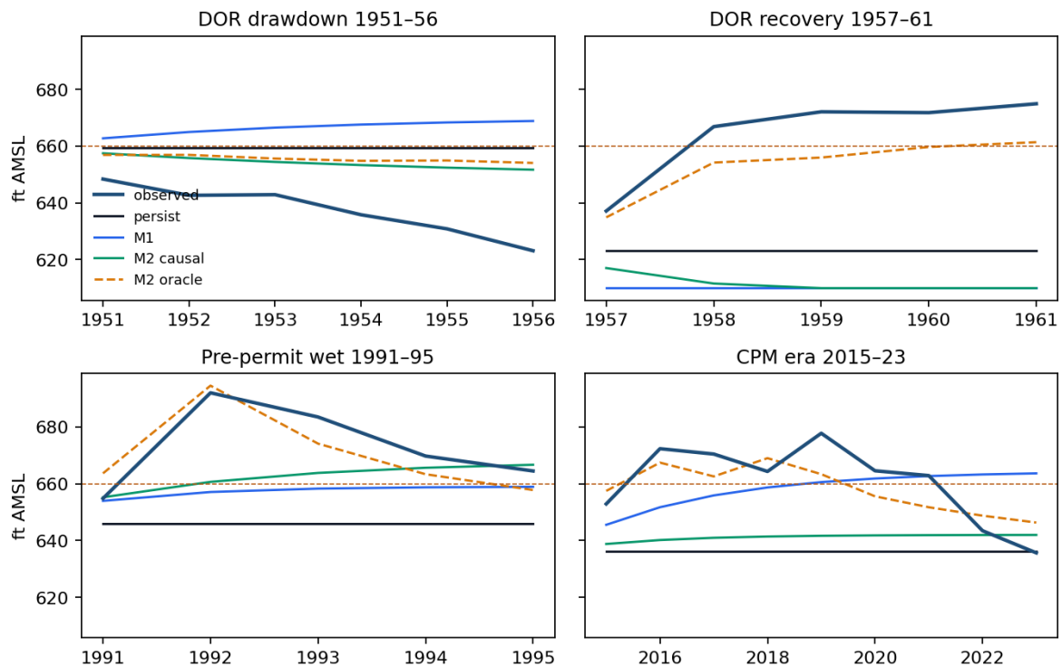
Figure 2. Multi-step forecasts from the end of each training window. The oracle (dashed) is diagnostic and uses realized future R, P.
