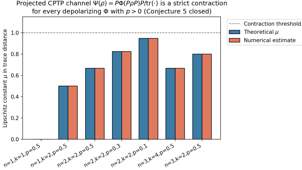
Fig. 2 Projected CPTP channel \Psi(\rho) = P\Phi(P\rho P)P/\text{tr}(\cdot) is a strict contraction in trace distance for every depolarizing \Phi with p > 0 . Bars show theoretical \mu (blue) and numerical Monte-Carlo estimate (rust) across configurations (n, k, p) ; all are below the contraction threshold \mu = 1 (dashed). At (n=2, k=2, p=0.1) the channel is weakly contractive ( \mu = 0.947 ); at (n=2, k=2, p=0.5) strongly contractive ( \mu = 0.667 ). Zeno self-reference resolution settled.
