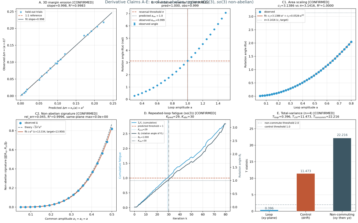
Fig. 4 Operational results for Claims A–E in the n = 4 non-abelian regime (structure group \text{SO}(3) ). (a) Claim A: three-dimensional held-out margin erosion; slope 0.9976, R^2 = 0.9983 . (b) Claim B: orientation-reversal amplitude 0.9992 against the predicted 1.0 (relative error 0.083%). (c) Claim C: single-plane holonomy-area scaling and the non-abelian commutator signature; the single-plane fit gives c_1 = 3.1386 (against \pi ) and c_2 = 0.0526 (against 0.0500), and the commutator fit gives c_{\text{comm}} = 13.33 against \sqrt{2}\pi^2 = 13.96 (relative error 4.5%). (d) Claim D: repeated-loop fatigue in \mathfrak{so}(3) via matrix increments F_k \mathfrak{l}_z ; K_{\text{pred}} = 29 and K_{\text{obs}} = 30 (relative error 3.4%). (e) Claim E: total-variance T -statistics with signed residuals; T_{\text{loop}} = 0.40 , T_{\text{ctrl}} = 11.47 , T_{\text{noncomm}} = 22.22 , with ratio T_{\text{noncomm}}/T_{\text{loop}} = 56 .
