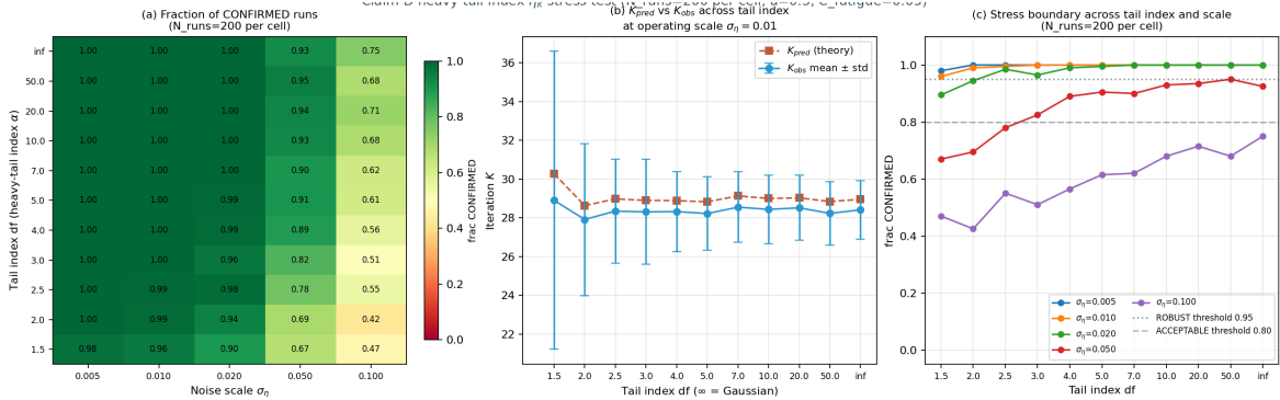
Figure 5: Heavy-tail index stress test of Claim D across the (\text{df}, \sigma_\eta) grid with 200 Monte-Carlo seeds per cell. (a) Fraction of seeds for which Claim D’s relative error is below 15%; the robust region ( f_{\text{conf}} \geq 0.95 ) covers the operating scale \sigma_\eta = 0.01 across all \text{df} \geq 2 . (b) K_{\text{pred}} and K_{\text{obs}} versus tail index at \sigma_\eta = 0.01 with mean \pm standard-deviation error bars; the two curves track within a relative error of at most 5%. (c) Stress boundary: f_{\text{conf}} versus \text{df} for each \sigma_\eta ; the robust threshold (0.95, dotted) and the acceptable threshold (0.80, dashed) bracket the operating regime. The infinite-variance boundary \text{df} = 2 is crossed smoothly.
