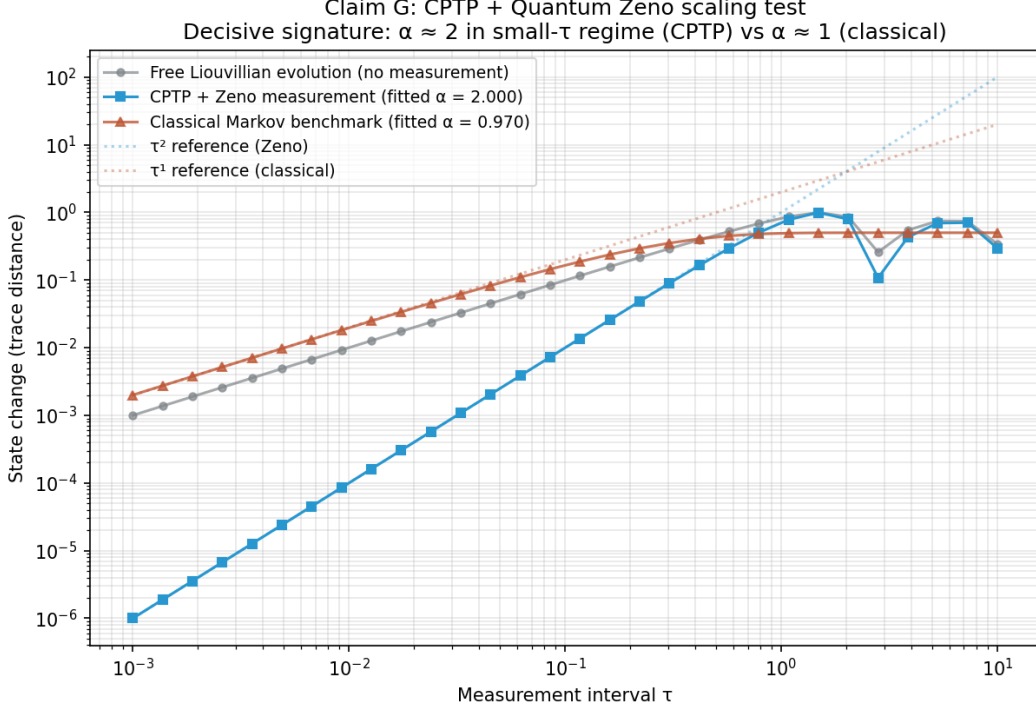
Figure 7: Claim G verdict. Log–log plot of state change (trace distance) versus measurement interval \tau . CPTP–Zeno points (squares) follow the \tau^2 reference line in the small- \tau regime; the fitted exponent is \alpha_{\text{Zeno}} = 1.9997 with R^2 = 1.0000 . Classical Markov points (triangles) follow the \tau^1 reference line; the fitted exponent is \alpha_{\text{cl}} = 0.9695 with R^2 = 0.9997 . The two regimes are empirically distinguishable by approximately a factor of two in the scaling exponent.
