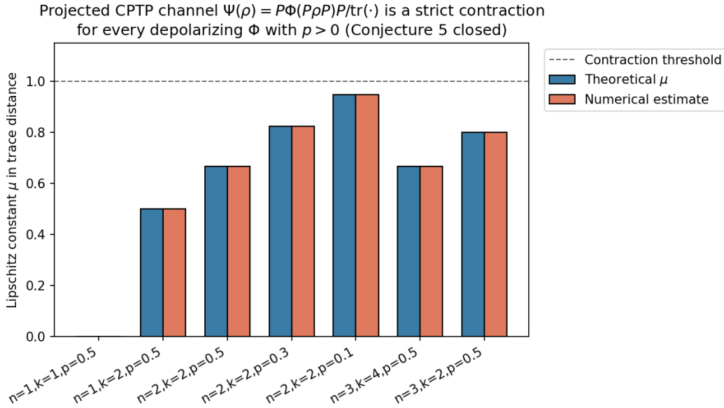
Figure 2: Projected CPTP channel \Psi(\rho) = P\Phi(P\rho P)P/\text{tr}(\cdot) is a strict contraction in trace distance for every depolarizing \Phi with p > 0 . Bars show theoretical \mu (blue) and numerical Monte-Carlo estimate (rust) across configurations (n, k, p) ; all are below the contraction threshold \mu = 1 (dashed). At (n=2, k=2, p=0.1) the channel is weakly contractive ( \mu = 0.947 ); at (n=2, k=2, p=0.5) strongly contractive ( \mu = 0.667 ). Zeno self-reference resolution settled.
