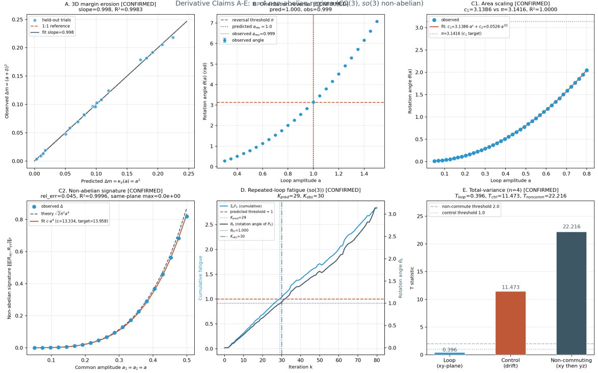
Figure 4: Operational results for Claims A–E in the n=4 non-abelian regime (structure group SO(3) ). (a) Claim A: three-dimensional held-out margin erosion; slope 0.9976, R^2 = 0.9983 . (b) Claim B: orientation-reversal amplitude 0.9992 against the predicted 1.0 (relative error 0.083%). (c) Claim C: single-plane holonomy-area scaling and the non-abelian commutator signature; the single-plane fit gives c_1 = 3.1386 (against \pi ) and c_2 = 0.0526 (against 0.0500), and the commutator fit gives c_{comm} = 13.33 against \sqrt{2}\pi^2 = 13.96 (relative error 4.5%). (d) Claim D: repeated-loop fatigue in \mathfrak{so}(3) via matrix increments F_k \mathfrak{l}_z ; K_{pred} = 29 and K_{obs} = 30 (relative error 3.4%). (e) Claim E: total-variance T -statistics with signed residuals; T_{loop} = 0.40 , T_{ctrl} = 11.47 , T_{noncomm} = 22.22 , with ratio T_{noncomm}/T_{loop} = 56 .
