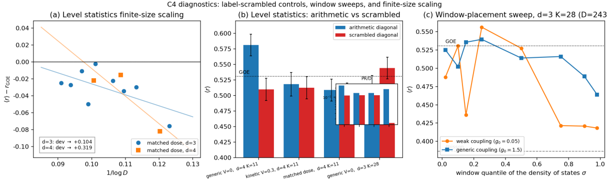
Figure 2: Audit-response controls for the C4/C5 numerics (Remark 3.17(f)–(g)). (a) Finite-size scaling of the level-statistics deviation \langle r \rangle - r_{\text{GOE}} against 1/\log D along the matched-dose ladders ( d = 3 circles, d = 4 squares; fits as lines): deviations shrink with D but the computed range does not settle the limiting value. (b) Arithmetic versus label-scrambled diagonal at four platforms ( \langle r \rangle with standard errors; inset: \text{PR}/D on a log scale): matched-dose \langle r \rangle is scramble-insensitive; the generic family is not, and the participation ratio collapses under scrambling. (c) Window-placement sweeps at d = 3 , K = 28 : the weak-coupling band (0.42–0.56) and the generic band (0.46–0.54) are both quantile-dependent; the generic compression sits at the band edges.
