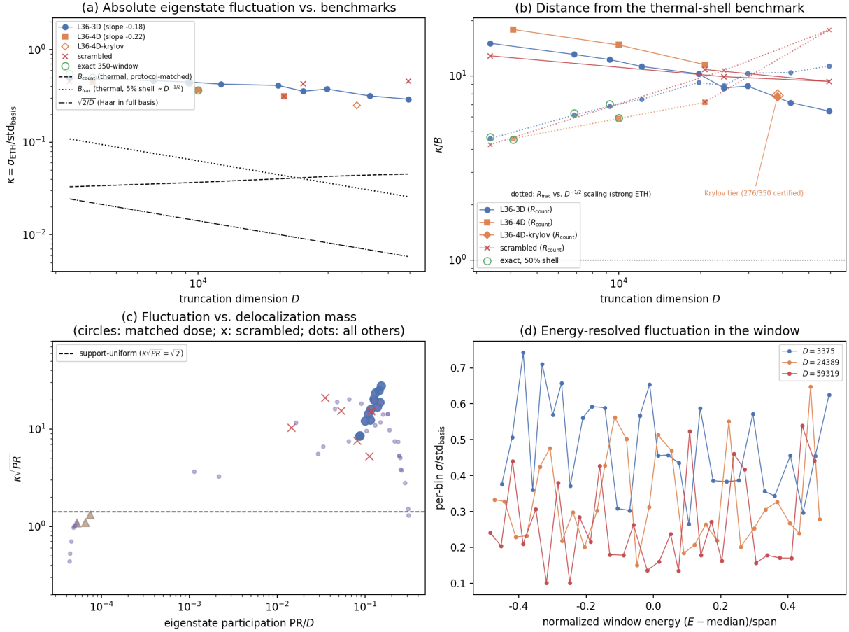
Figure 3: Absolute eigenstate-fluctuation scaling at matched dose (Remark 3.11(h)–(i)). (a) \kappa = \sigma_{\text{ETH}}/\text{std}_{\text{basis}} versus truncation dimension (window values, exact 350-state selections, label-scrambled controls, and the factorization-free Krylov-tier point at D = 3.84 \times 10^4 , open diamond: 276 of 350 pairs certified) against the calibrated benchmarks: the protocol-matched shell benchmark B_{\text{count}} , the fixed-fraction B_{\text{frac}} \propto D^{-1/2} (the strong-ETH scaling), and the Haar-in-full-basis level \sqrt{2/D} . (b) Distance from the benchmarks: \kappa/B_{\text{count}} (solid) falls slowly; \kappa/B_{\text{frac}} (dotted) grows. (c) \kappa\sqrt{\text{PR}} versus eigenstate participation across all computed window configurations (matched dose: circles; scrambled: crosses; all others: dots), against the support-uniform level \sqrt{2} : the fluctuation sits 10–30 times above it and grows with D . (d) Energy-resolved within-window fluctuation at three scales.
