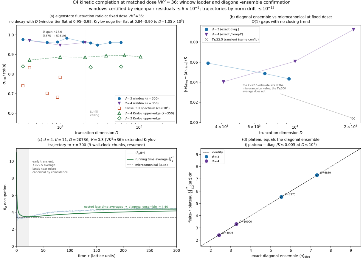
Figure 2: Matched-dose ( VK^2 \approx 36 ) numerics for the kinetic completion (Remark 3.11(d)–(e)). (a) Eigenstate fluctuation ratio \sigma_{\text{ETH}}/\text{std}(a) versus truncation dimension: window values (filled) and exact full-spectrum values (open); no decay across a factor 17.6 in D . (b) Distance of the diagonal ensemble from the microcanonical value, normalized by K : O(1) gaps with no closing trend; the T \leq 22.5 estimate (cross) is a transient that coincides with the microcanonical value. (c) The d = 4 , K = 11 , D = 20736 , V = 0.3 trajectory extended to \tau = 300 : observable, running time average, nested late-time averages (diagonal-ensemble estimate \approx 4.40 ), microcanonical line, and the early transient. (d) Finite- T plateau versus exact diagonal ensemble at D \leq 10^4 (identity line).
