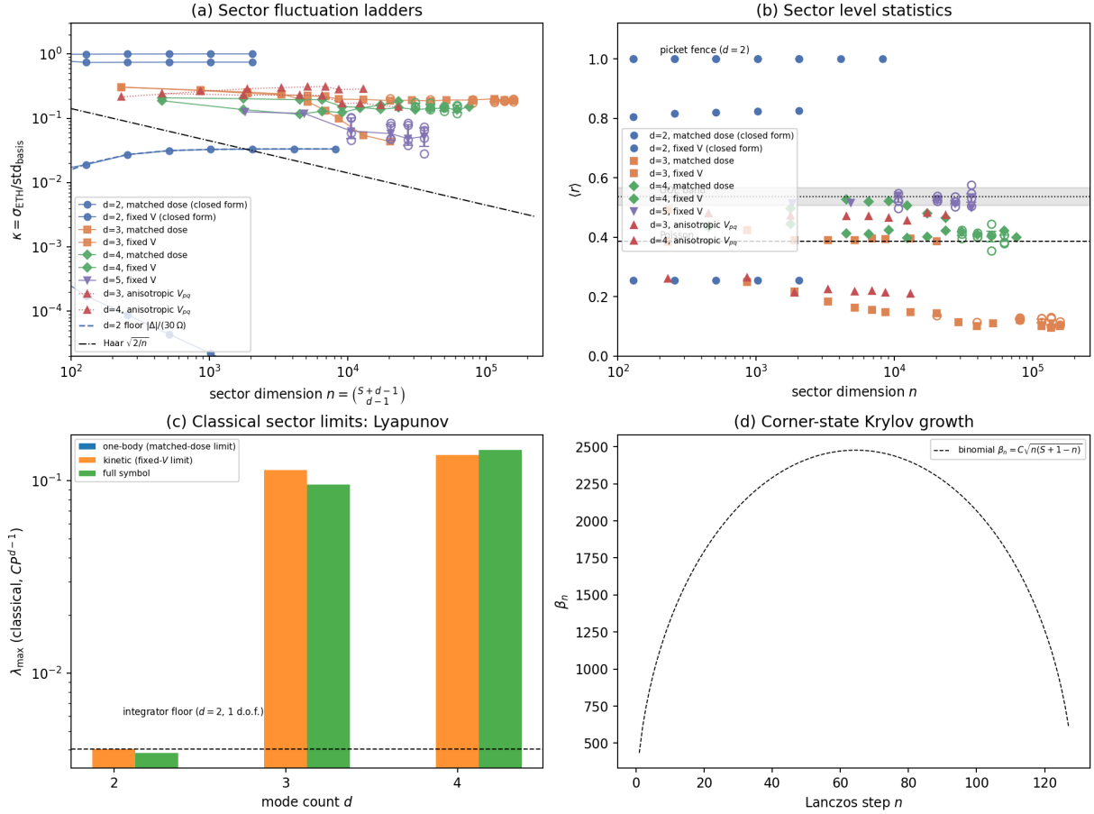
Figure 1: Occupation-sector falsifier ladders (Remark 3.12(1)). (a) The fluctuation ratio \kappa = \sigma_{\text{ETH}}/\text{std}_{\text{basis}} of the mode-1 occupation against the sector dimension n = \binom{S+d-1}{d-1} : matched-dose and fixed- V families at d = 2 (closed form, with the analytic floor |\Delta|/(30\Omega) ), d = 3 , d = 4 , the d = 5 fixed- V family, and \pm 30\% anisotropic controls, against the Haar benchmark \sqrt{2/n} (filled points: the seed-7 ladders; open circles: replicate controls; error bars: realization means with between-realization spread over the amendment tail rungs). (b) Level statistics \langle r \rangle against n with the Poisson and GOE references and the GOE band; the d = 2 picket fence sits at \langle r \rangle = 1 at every scale. (c) Benettin exponents of the classical sector limits on \mathbb{C}P^{d-1} : the one-body (matched-dose) flow is integrable at every d , the kinetic (fixed- V ) flow is chaotic for d \geq 3 . (d) Corner-state Lanczos coefficients \beta_n ; the d = 2 sequence is the binomial law exactly.
