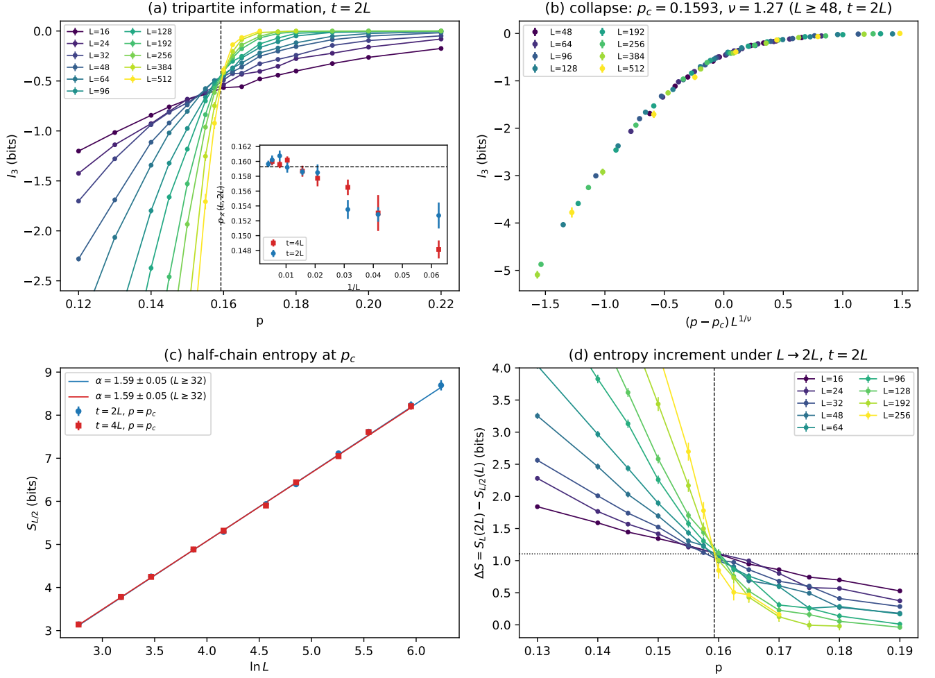
FIG. 1. Quenched Clifford transition, t = 2L . (a) I_3(p) for L = 16 –512; dashed line p_c = 0.1593 from the collapse in (b); inset: crossings p_{\times}(L, 2L) (PCHIP estimator) against 1/L at t = 2L (circles) and t = 4L (squares). (b) Collapse I_3 = F((p - p_c)L^{1/\nu}) , L \geq 48 , |x| \leq 1.6 shown. (c) S_{L/2} at p_c (spline-interpolated in p ) against \ln L at t = 2L and 4L with the L \geq 32 fits. (d) Entropy increment \Delta S = S_{L/2}(2L) - S_{L/2}(L) ; at p_c it equals \alpha \ln 2 (dotted) independently of L .
