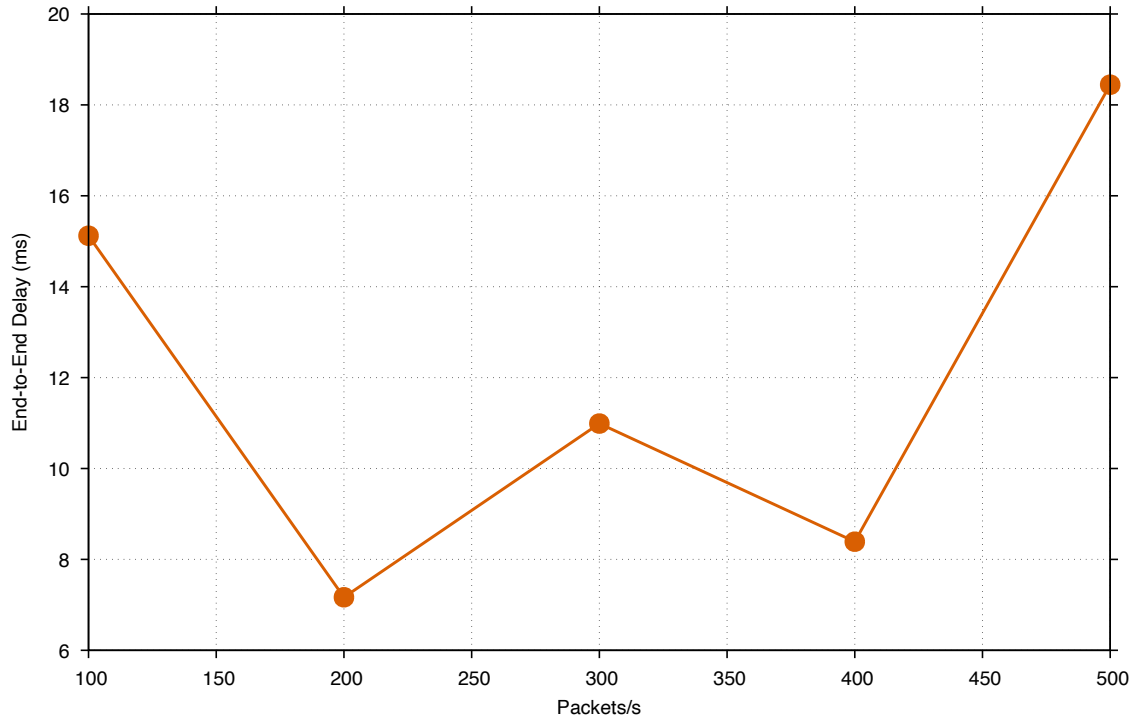
Wired Bolt End-to-End Delay (ms) vs Packets/s
