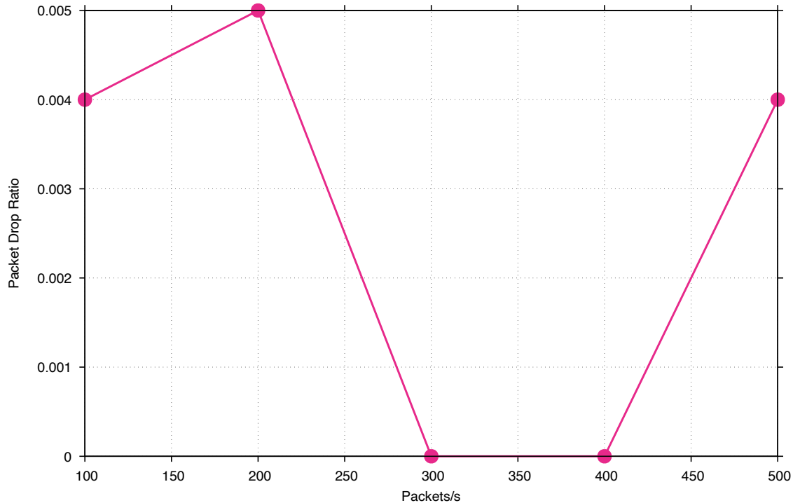
Wired Bolt Packet Drop Ratio vs Packets/s
