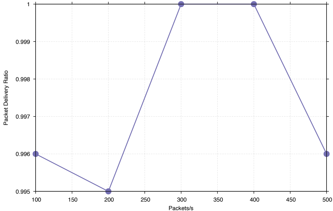
Wired Bolt Packet Delivery Ratio vs Packets/s
